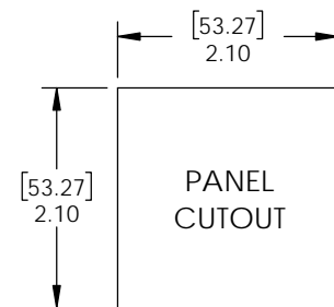
-2/-4 Configurations
