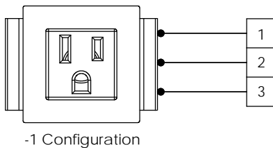
-1 Configuration
