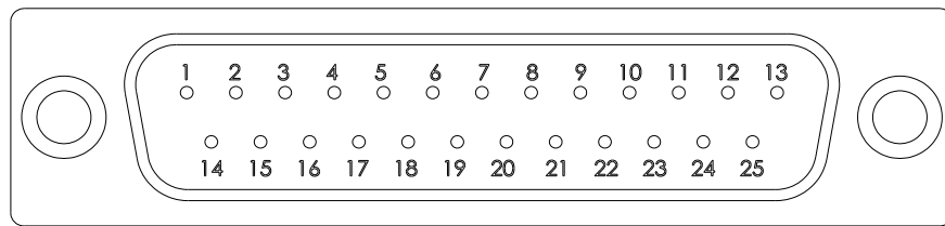
FIGURE 3.3 REAR VIEW OF 25-PIN D-SUB CONNECTOR (J1)
